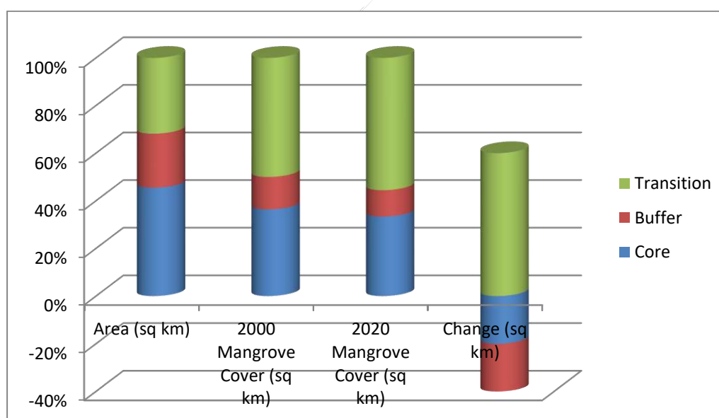
Figure 2: Changes in Specific Mangrove Types
