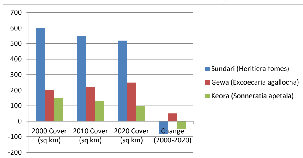
Figure 3: Changes in Specific Mangrove Types
