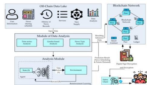
FIGURE 1. Block diagram of the proposed fake news detection approach.
