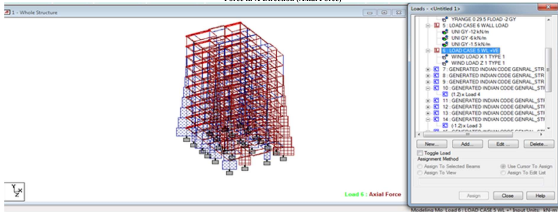
Force in X Direction (Axial Force)
