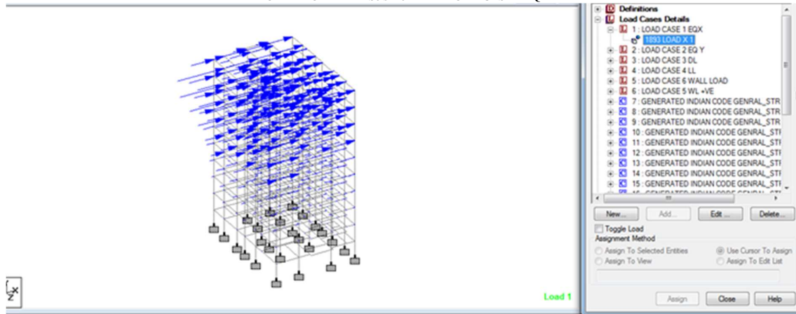
LOAD 1 LOADTYPE Seismic TITLE LOAD CASE 1
