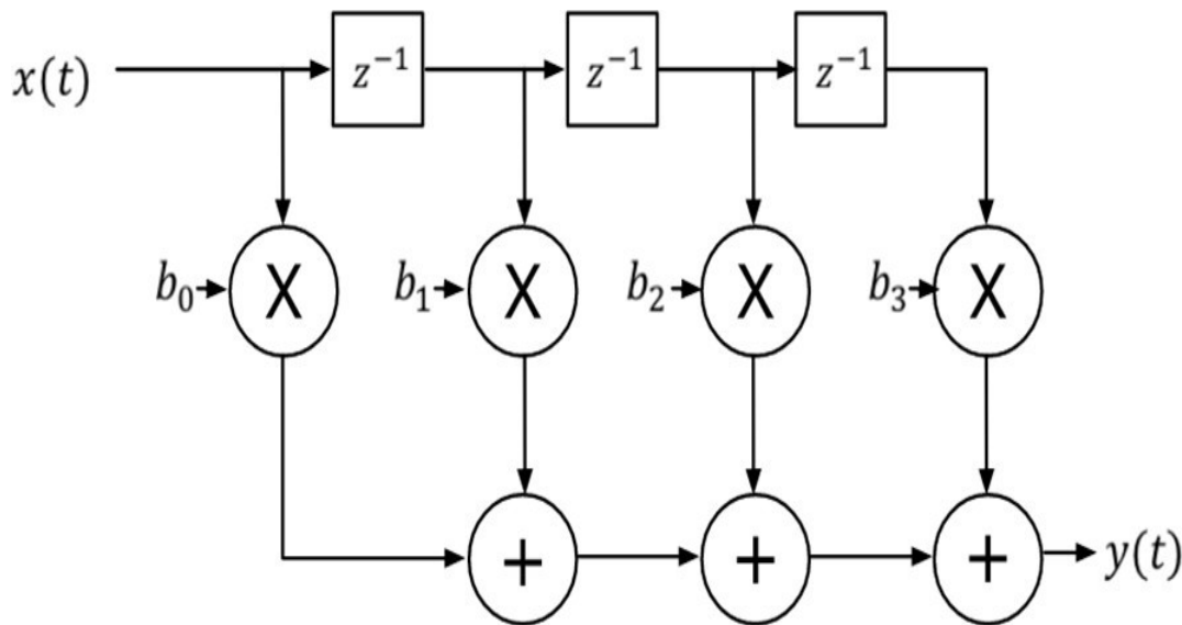
Fig 1:Block Diagram for 4-Tap FIR Filter
