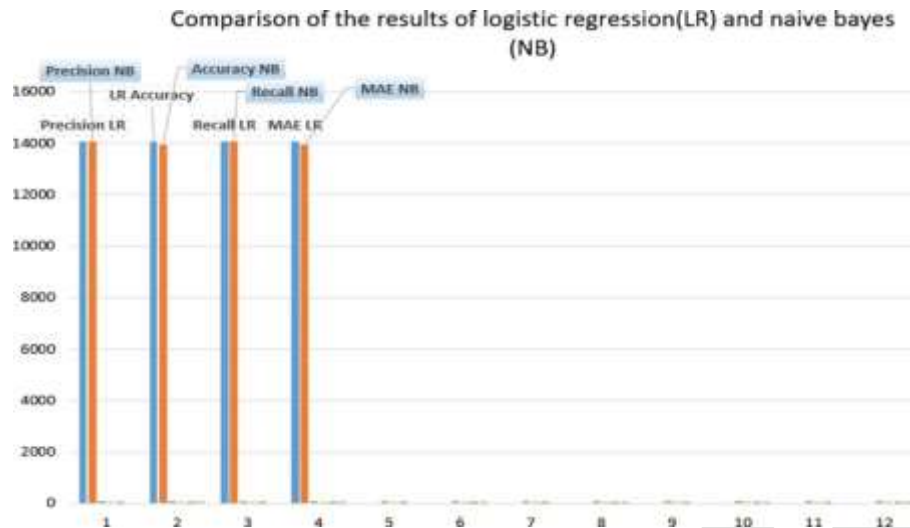
Fig. 9 Graphical comparison of the logistic regression and naive bayes algorithm
