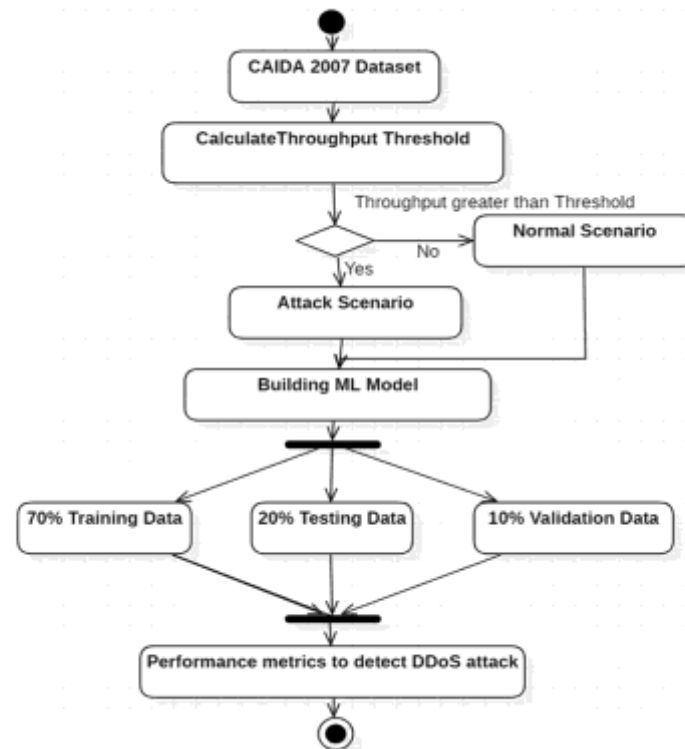
Fig. 2 Activity Diagram for experimental model
